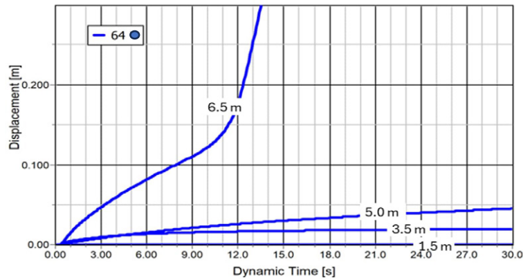
Figure 18: Dynamic displacement at crest (RL 64 m) vs. excavation depths
