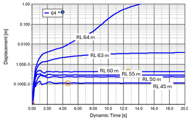
Figure 13: Dynamic displacement vs. phreatic line elevation
