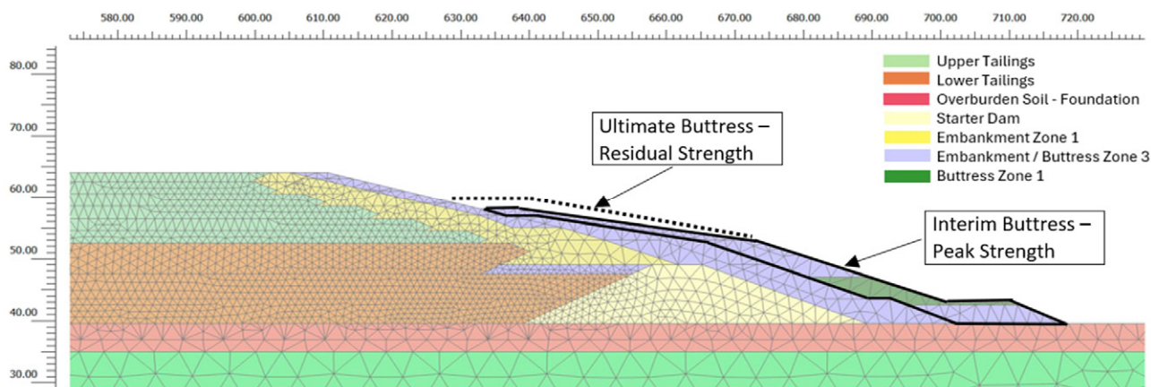
Figure 1: Typical cross section – TSF Cell 2 at MRM
