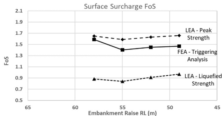
Figure 23: FoS vs embankment RL - surface surcharge mechanism
