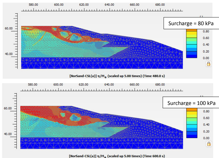
Figure 10: Evolution of softening zones within increasing surface surcharge
