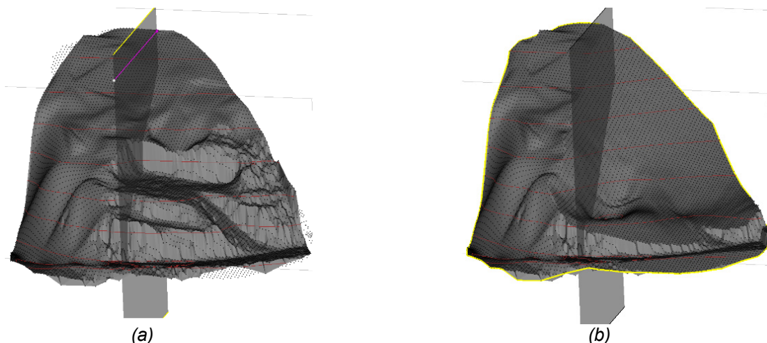
Figure 5. (a) Current slope; and (b) GW / CV interface, showing cross-section line
