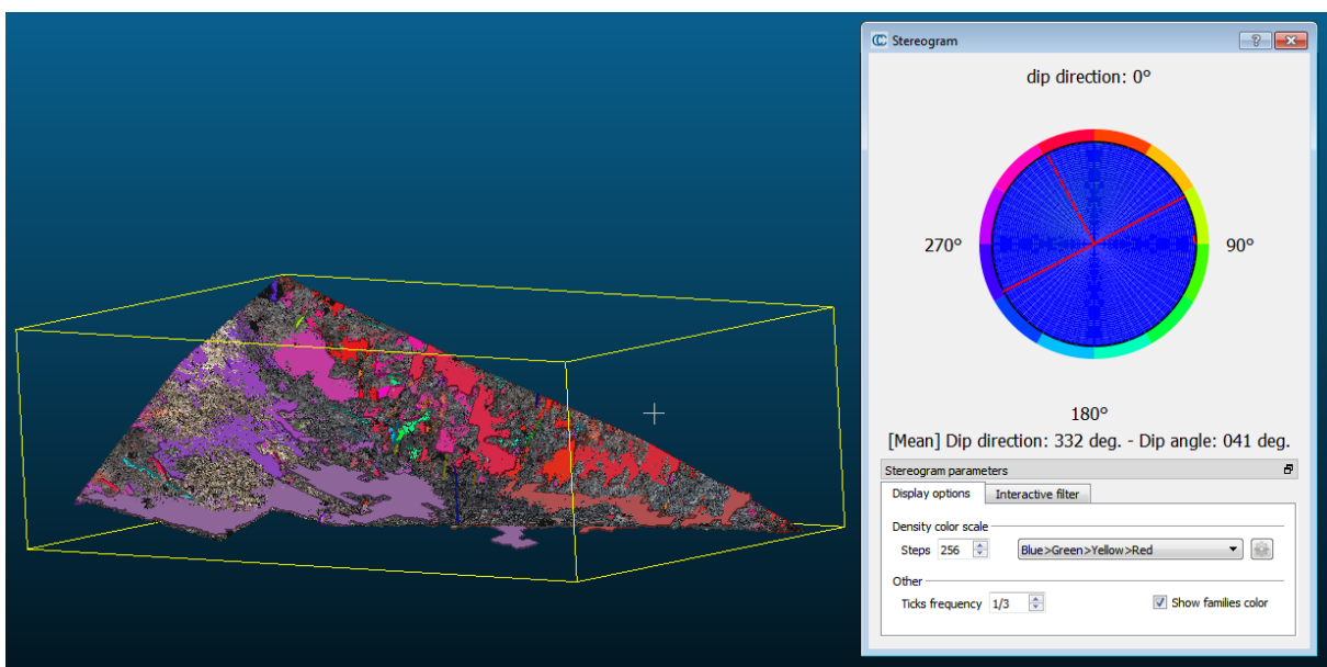
Figure 3. CloudCompare fracture orientation and stereonet
