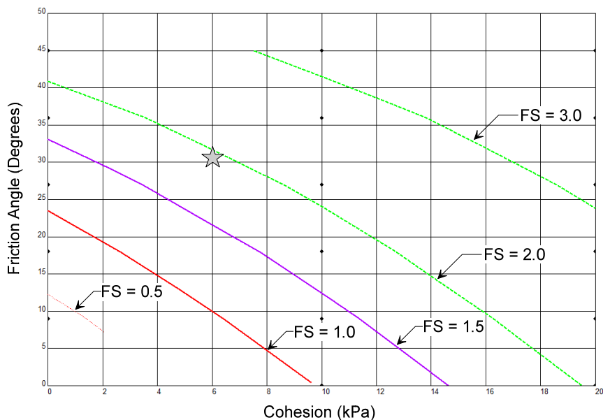
Figure 7. Cross plot of friction angle versus cohesion for a range of factors of safety. The star indicates Davidge (2007) parameters.
