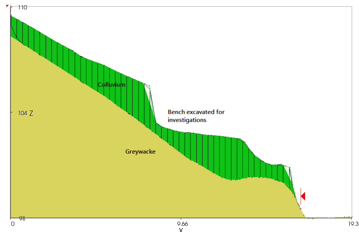
Figure 6. Cross-section showing slope failure controlled by greywacke/colluvium contact
