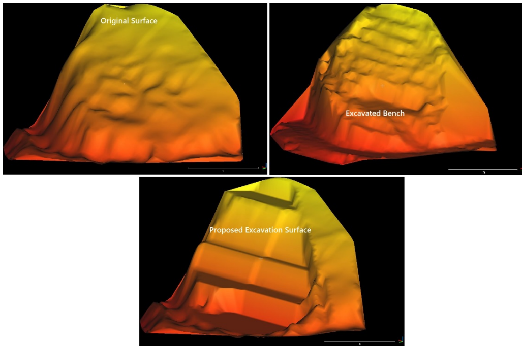
Figure 4. 'Original', 'current' (showing the bench excavated for investigation) and 'proposed' ground surfaces
