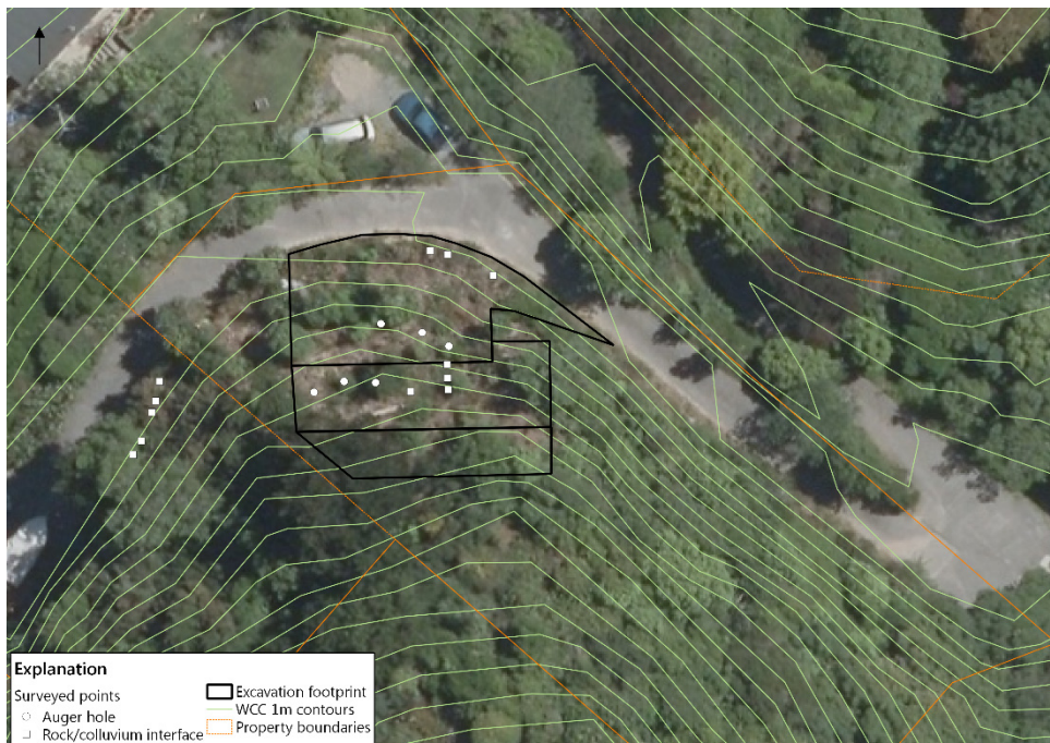
Figure 1. Topography, auger holes and surveyed rock/colluvium contacts
