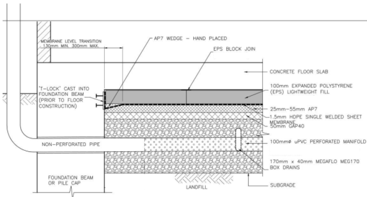
Figure 3. Typical details of Area 1 passive ventilation
