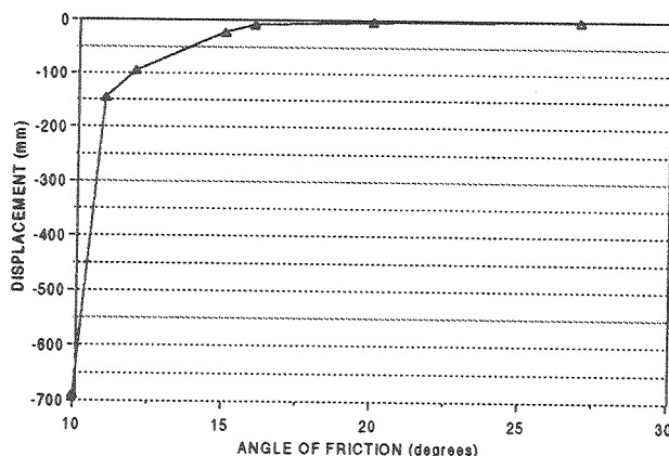
Figure 7 Predicted displacement at toe of dune
