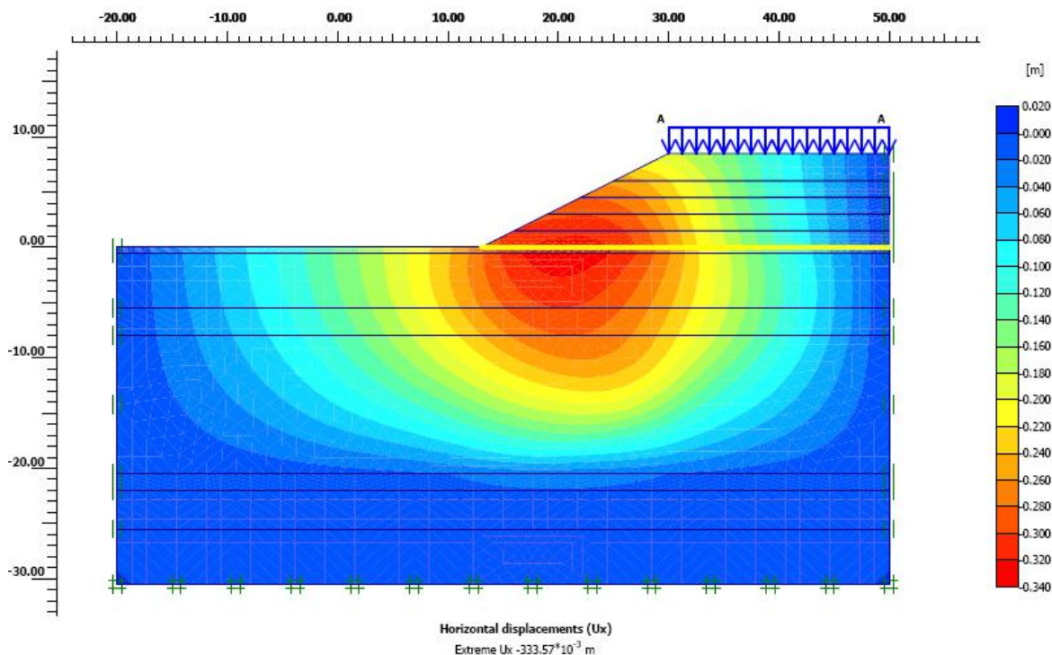
Figure 11: Results of 2D Finite Element analysis on BR25A & B (reinforced sections).
