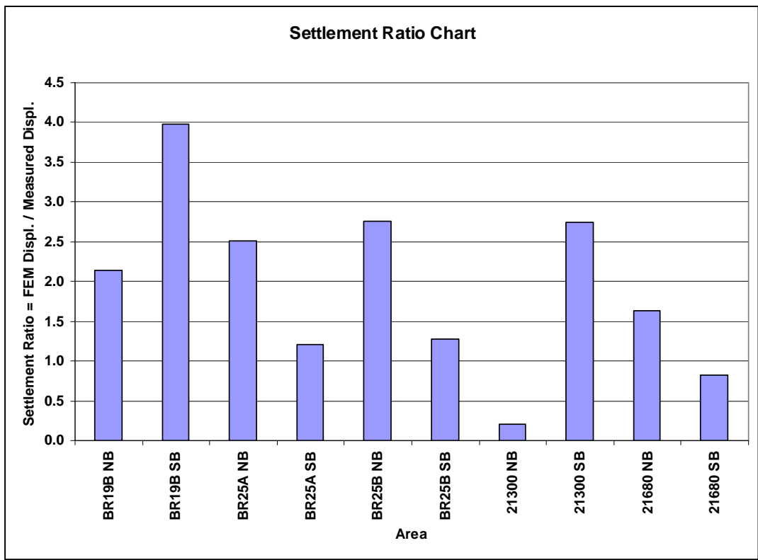
Figure 14: FEM Horizontal Displacements Vs Field Measured Horizontal Displacements.
