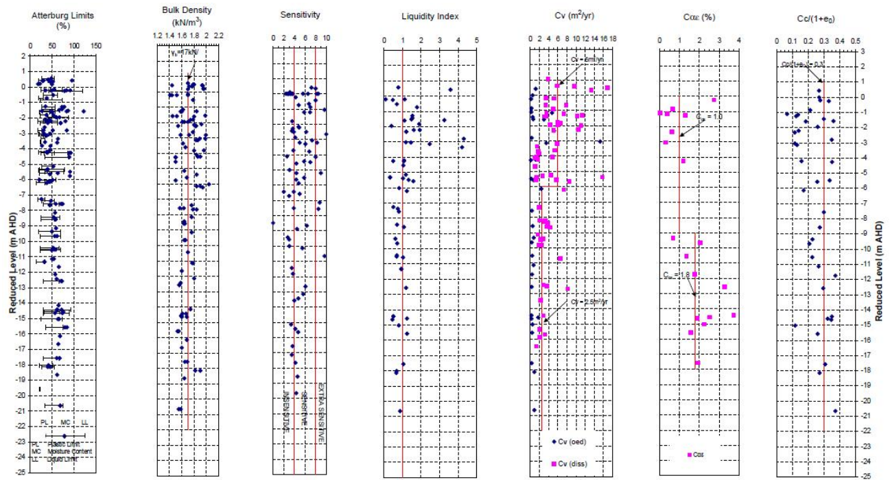
Figure 3: General soil properties from laboratory tests at Airport Interchange area (Coffey Report, 2007).
