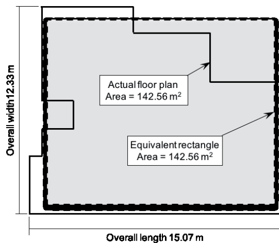
Figure 6 - Equivalent rectangular floor plan
