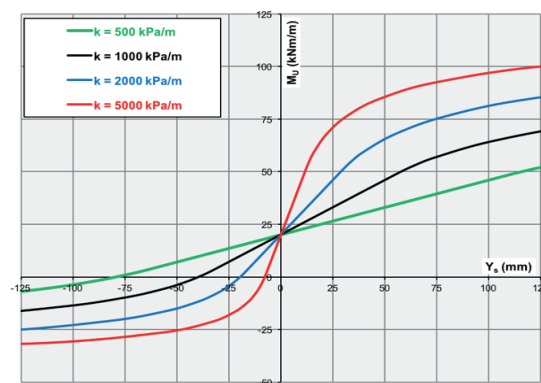
Figure 3. Effect of soil stiffness on slab design
