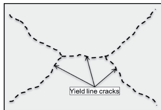
Figure 1. Fully developed yield line crack pattern
