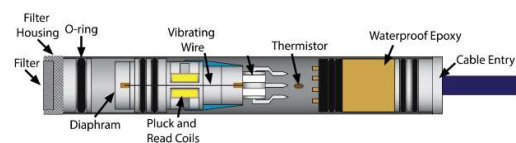
Figure 1. Typical Vibrating Wire Piezometer
