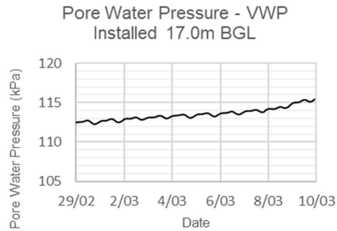
Figure 6. Pore Water Pressure data
