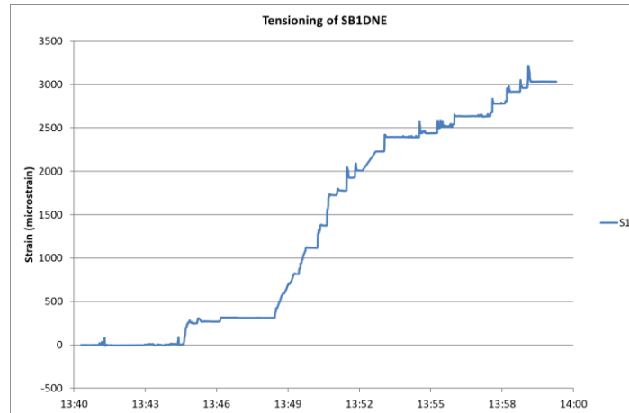
Figure 9: Tensioning S_B1_DNE1
