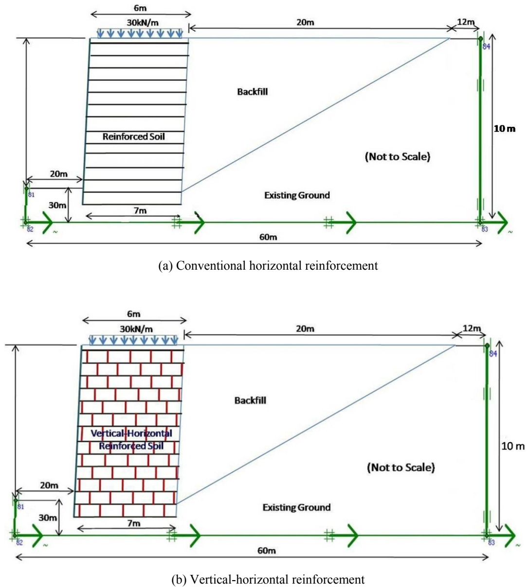
Figure 3: General models of the reinforced soil wall, (a) a horizontally reinforced wall without vertical reinforcement and (b) a reinforced wall with vertical and horizontal reinforcement
